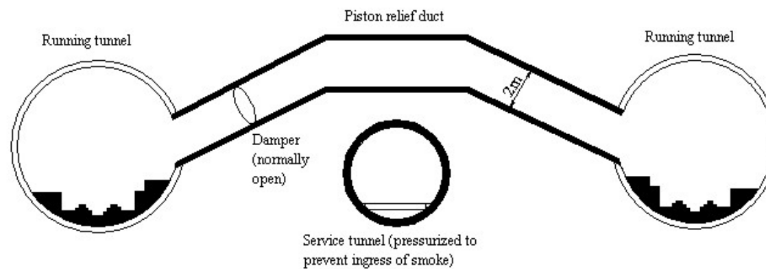
b) Section through tunnel at piston relief duct position
