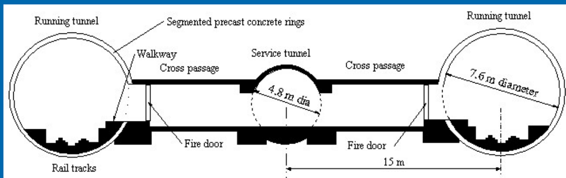
a) Section through tunnel at cross passage position
